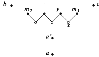
Fig. 2.13: A value of the multimedian in a graph
