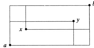
Fig. 3.1: the inversion law
