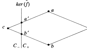
Fig. 2.4: the kernel of a norm-functional
