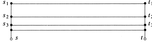
Fig. 3.3: the (2,2)-IP is not inherited by the completion
